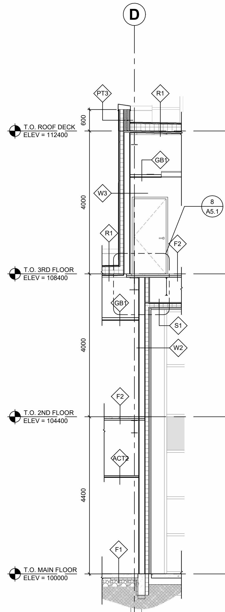
3 WALL SECTION A3.3 SCALE = 1 : 50
