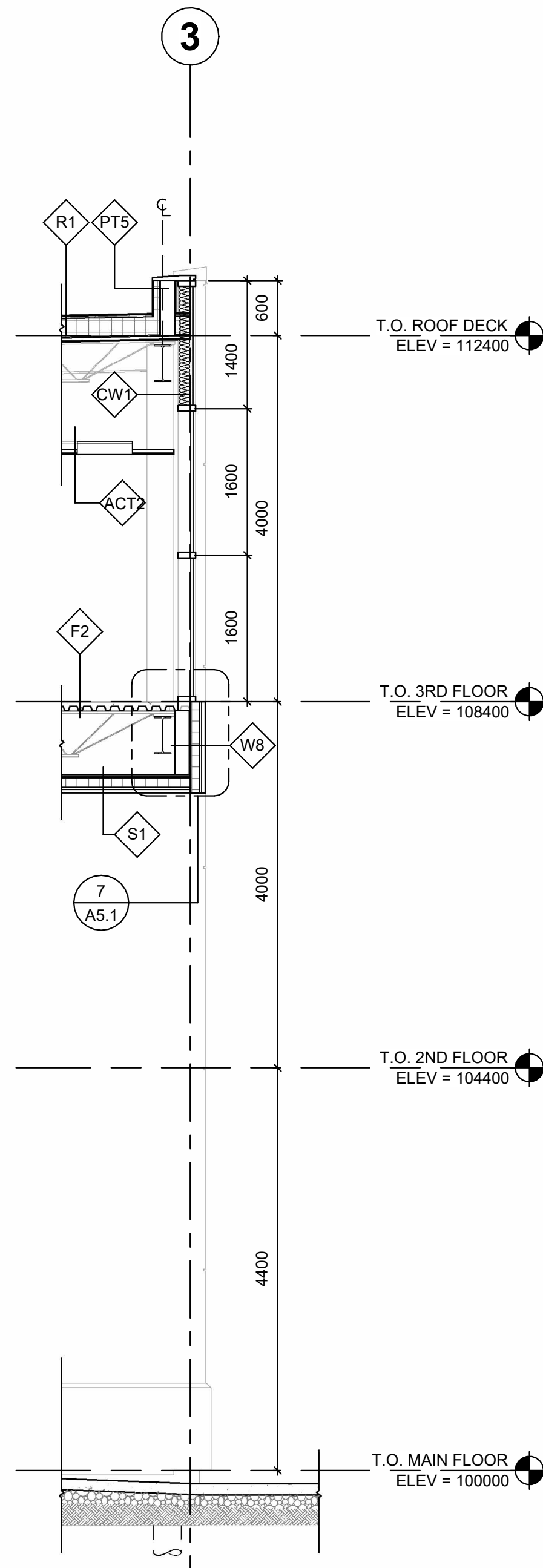
2 WALL SECTION A3.4 SCALE = 1 : 50
