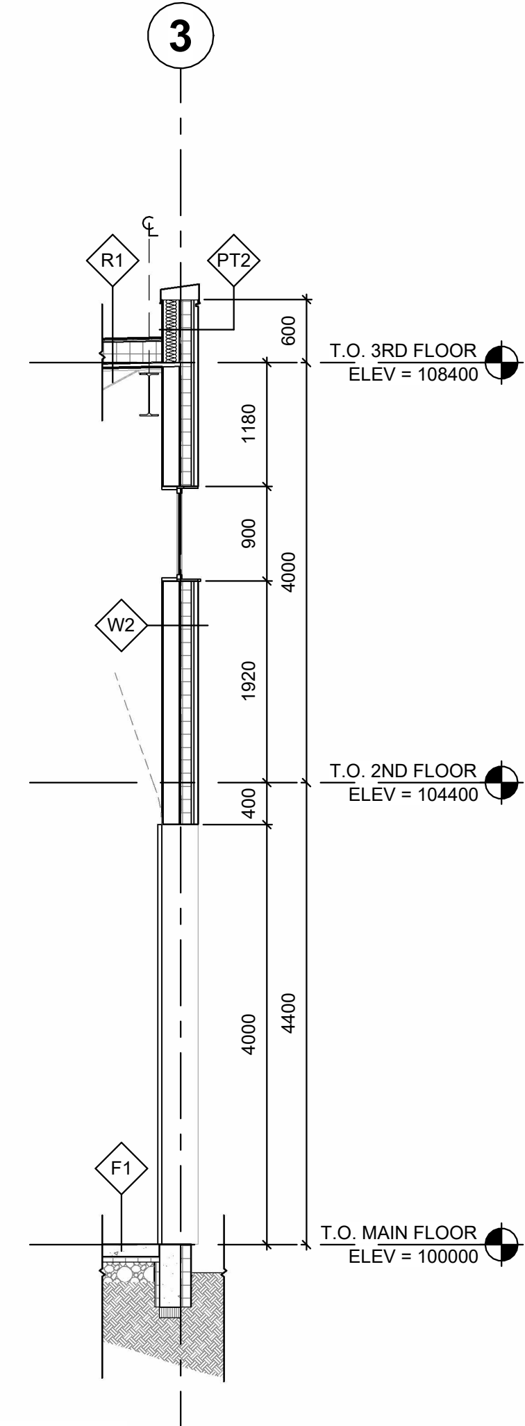
5 WALL SECTION
