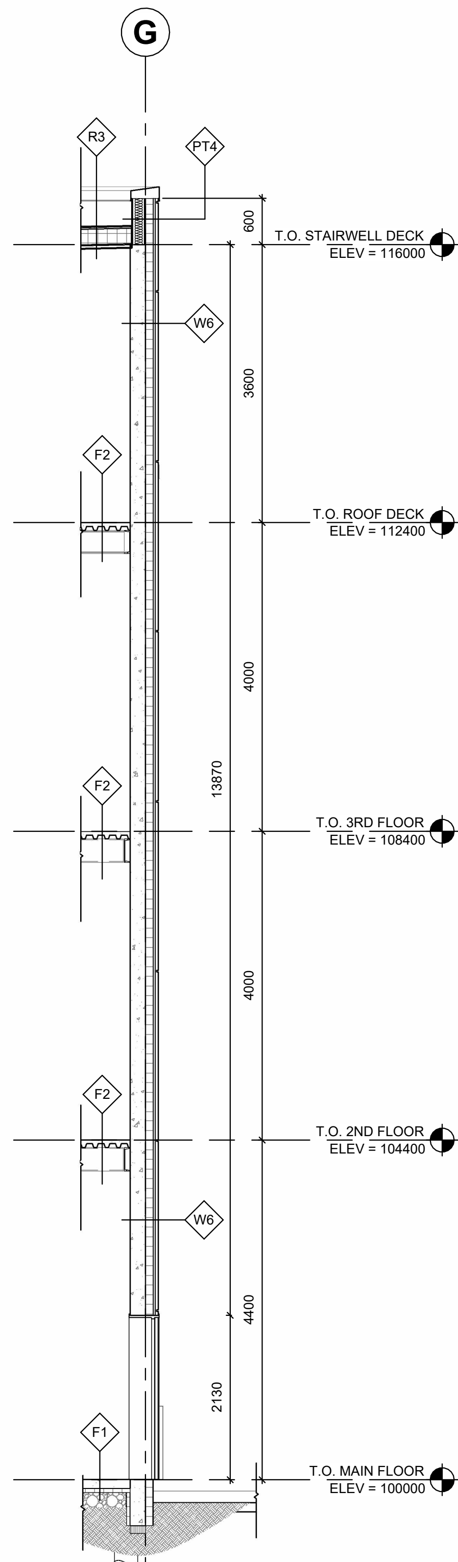
1 WALL SECTION A2.1 SCALE = 1 : 50
